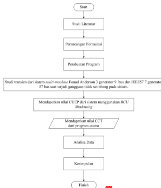
Gambar 2. Diagram Alir Perhitungan Critical Clearing Time
