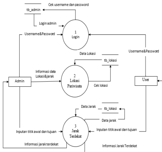
Gambar 3. DFD level 1
