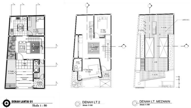
Gambar 2. Denah Recycle House (Avys, 2017)
