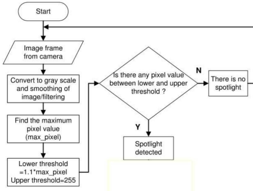
Figure 2. The laser spot detection algorithm proposed by [14].
