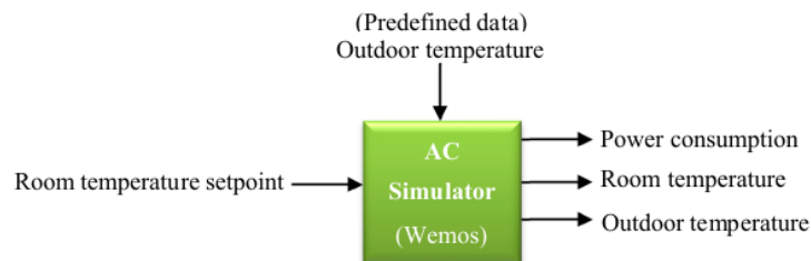
Figure 7. Block diagram of the AC simulator.
