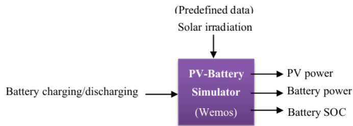
Figure 10. Block diagram of the PV-battery simulator.
