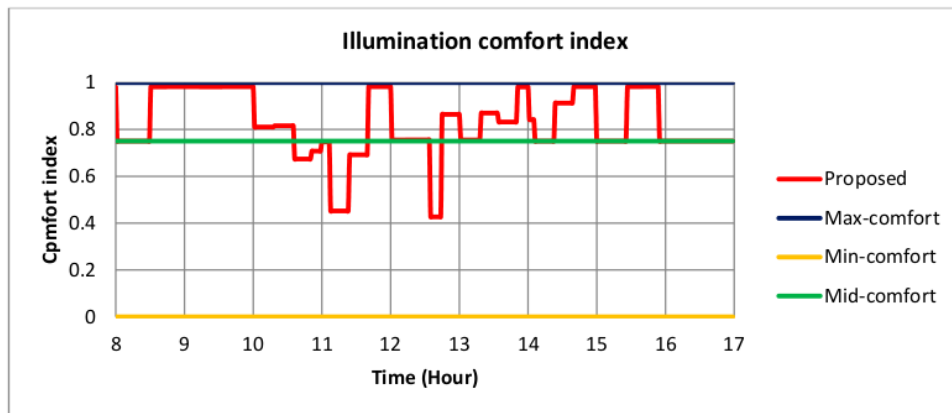
Figure 20. Illumination comfort index in the office room.
