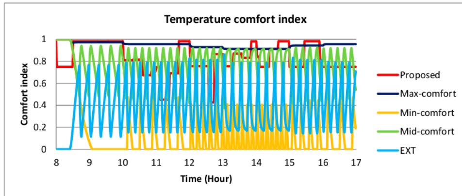
Figure 19. Temperature comfort index in the office room.
