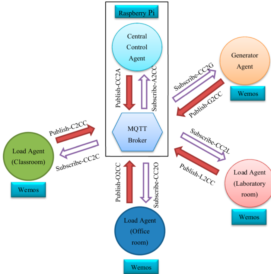
Figure 11. MQTT protocol configuration.
