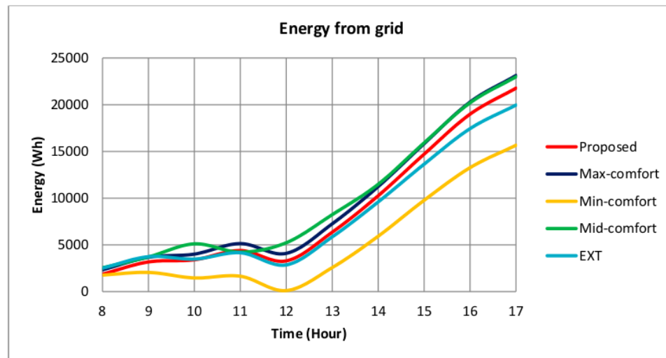
Figure 21. Energy extracted from the grid.
