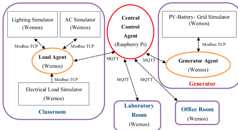
Figure 1. Architecture of the proposed system.
