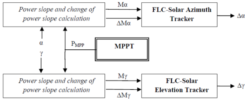
FIGURE 2. Configuration of FLC solar tracker
