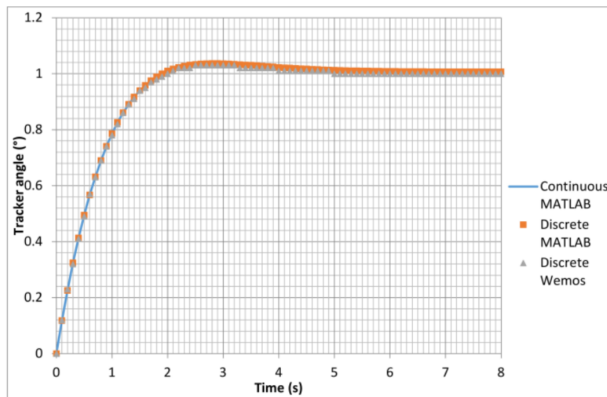
Figure 7. Response times of solar tracker models.
