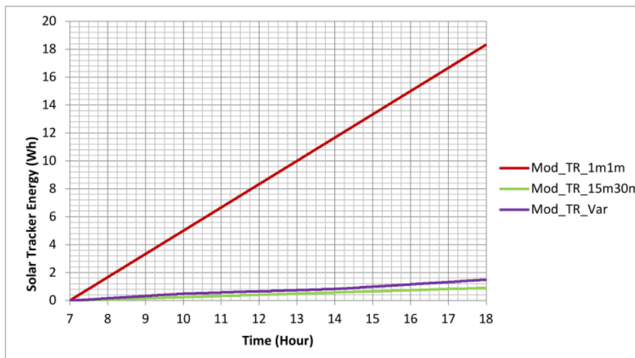
Figure 14. Energy consumed by solar tracker.
