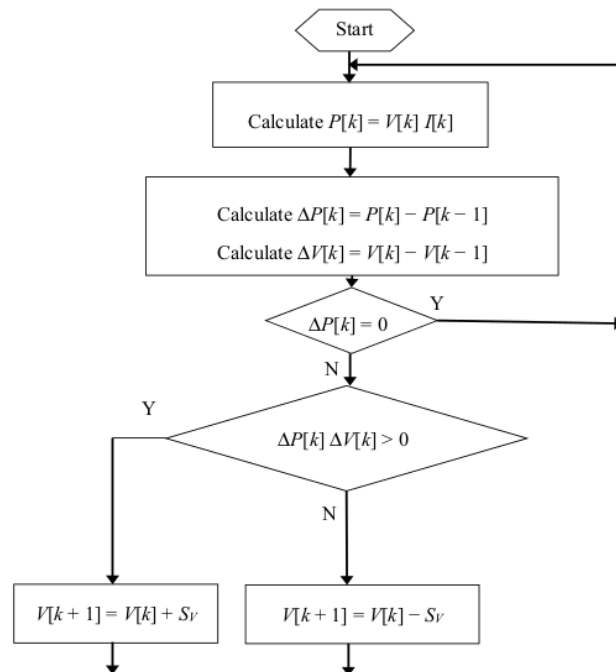
Figure 4. Flowchart of Perturb and Observe (P&O) algorithm [4].
