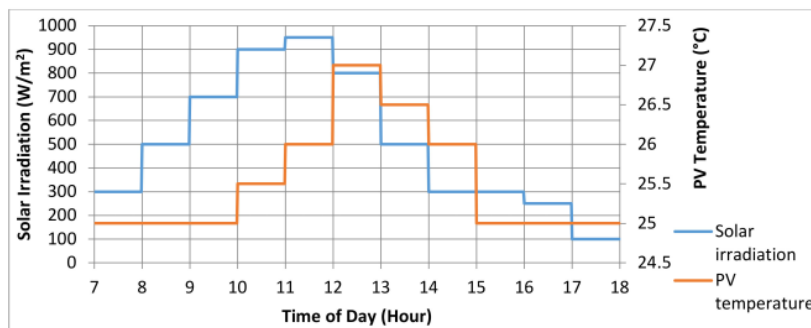
Figure 10. Profiles of solar irradiation and PV temperature.
