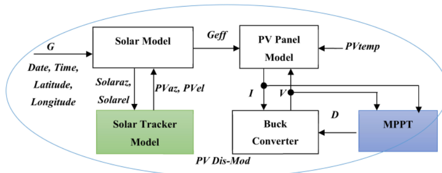
Figure 1. Configuration of the proposed discrete photovoltaic (PV) model. G : solar irradiation; G_{eff} : effective solar irradiation; PVtemp : PV temperature; Solaraz : solar azimuth; Solarel : solar elevation; PVaz : PV panel azimuth; PVel : PV panel elevation; V : PV voltage; I : PV current; D : duty cycle of DC-DC converter; PV Dis-Mod: Discrete PVmodel.
