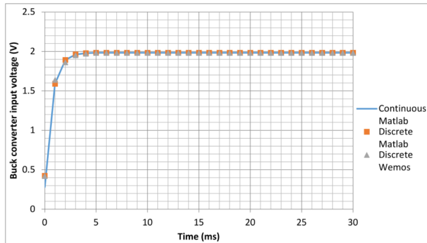
Figure 8. Response times of buck converter models.
