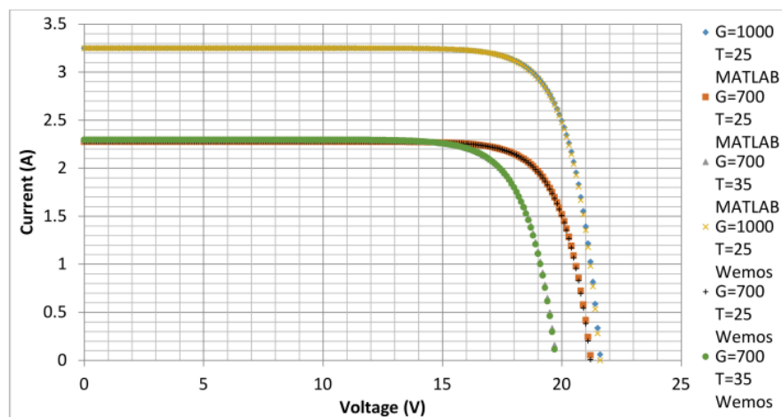
Figure 6. PV current and voltage characteristic of models.
