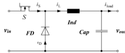
Figure 5. Buck converter model [2].
