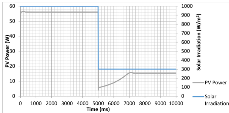
Figure 9. Response time of MPPT algorithm.
