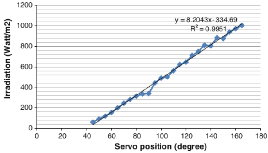
Fig. 25.4 Linearity between servo position and irradiation level
