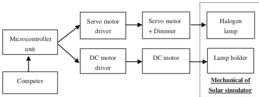
Fig. 25.2 Block diagram of solar simulator
