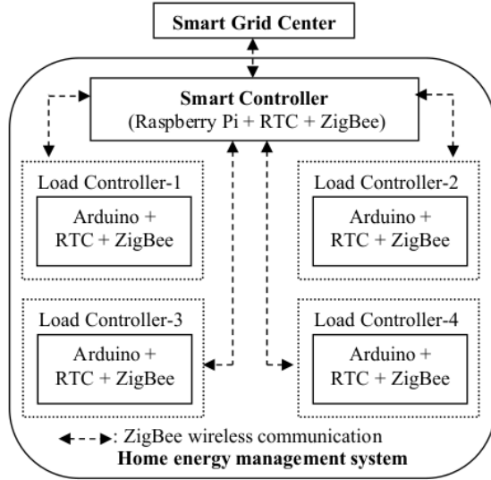
Fig. 1. Proposed HEMS.
