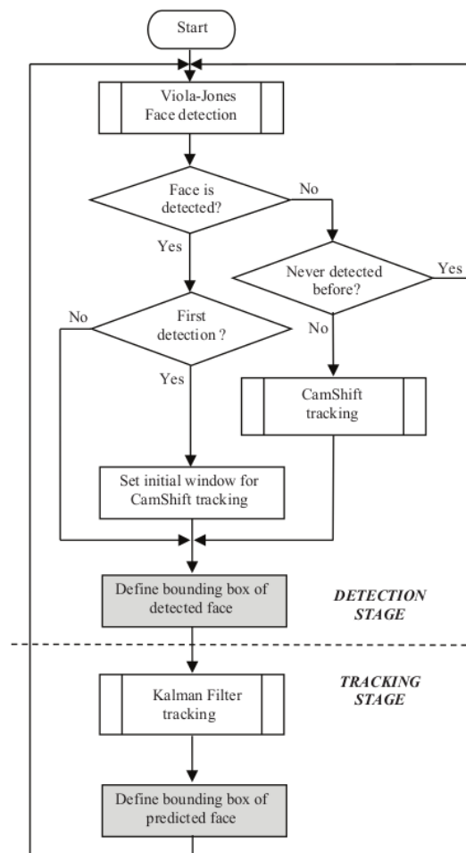
Fig. 1. Proposed face detection and tracking.
