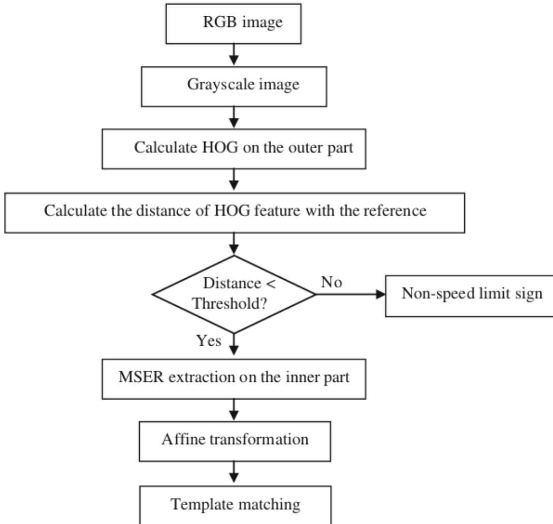
Fig. 1. Flowchart of proposed system
