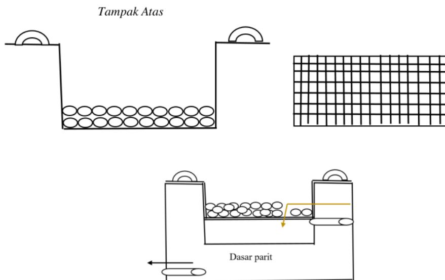
Gambar 12. Gambaran IPTEK (Alat Filter Plat dan Wiremesh)
