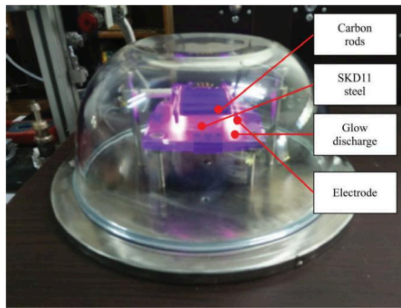
Fig. 2. Plasma sputtering process on the vacuum chamber
