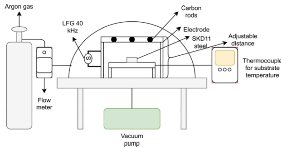
Fig. 1. Scheme of the plasma sputtering system
