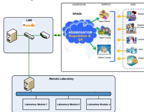
Figure 3. Integration of SPADA, LMS and Remote Lab
