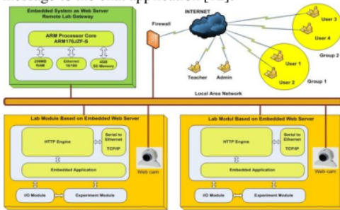
Figure 2. Remote laboratory architecture [12]
