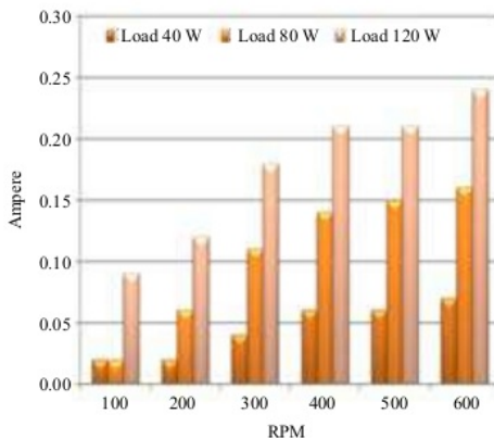
Fig. 9: Comparison graph of multi rotor and stator generator currents
