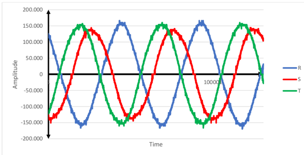
Figure 4. Three phase wave output from axial generator at 21 Hz frequency
