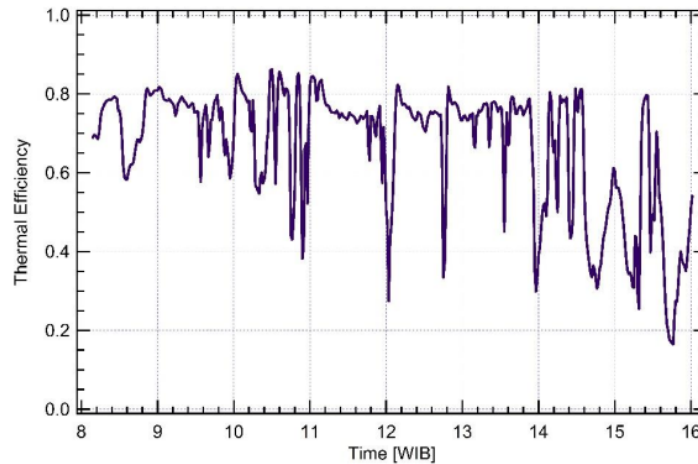
Figure 5. Thermal efficiency of the solar collector
