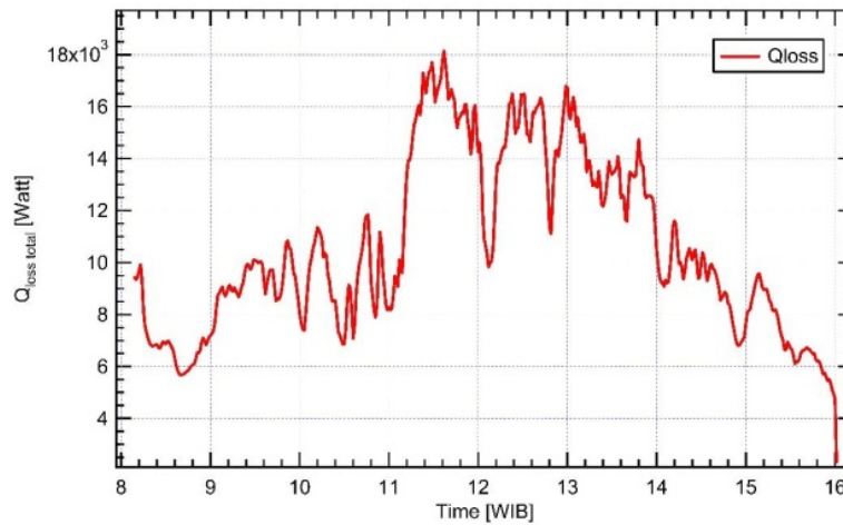
Figure 3. Heat loss from the collector
