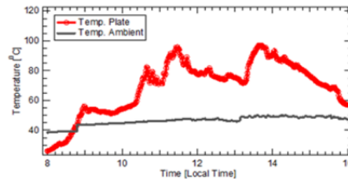
Figure 6. Heat Loss on Collectors
