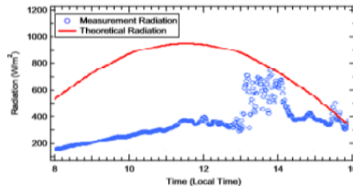
Figure 5. Theoretical radiation and measurement radiation
