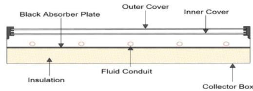
Figure 3. Basic Flat-Plate Solar Collector
