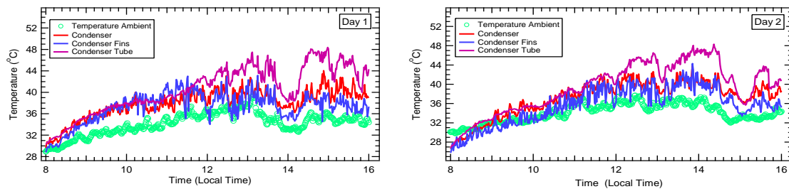
Figure 4. Environmental Temperature and Condenser
