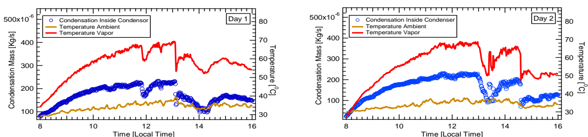
Figure 5. Condensation mass
