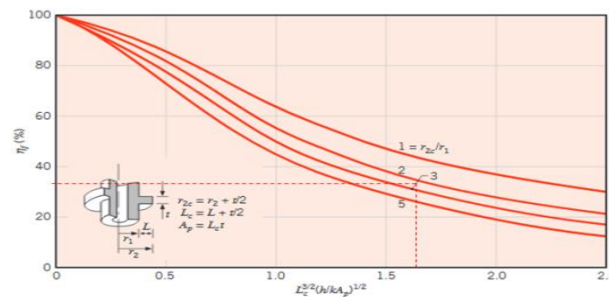
Figure 6. Fin Effectiveness [14]
