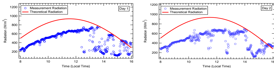
Figure 3. Theoretical Radiation and Radiation Measurements
