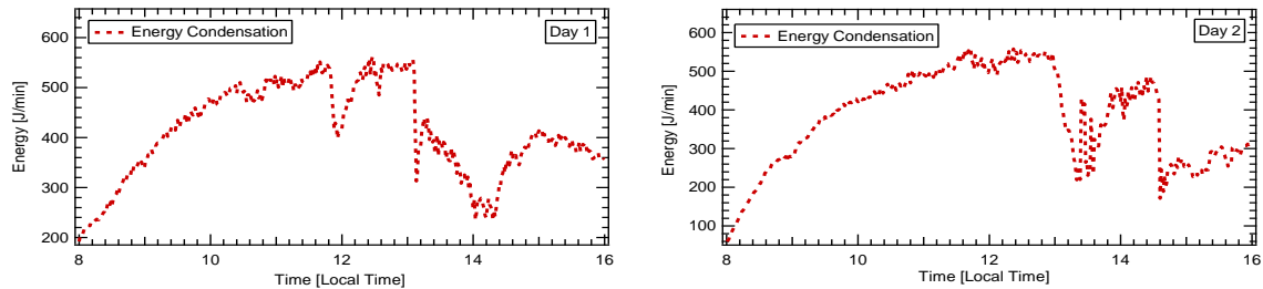
Figure 7. Energy for the Condensation Process
