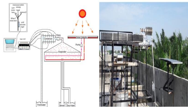
Figure 1. Desalination Experiment Tool and Desalination Scheme
