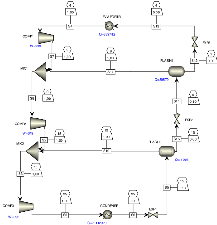
Figure 3. Three-stage vapour compression cycle in Aspen-Plus
