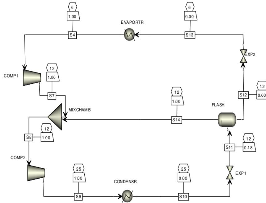
Figure 2. Two-stage vapour compression cycle in Aspen-Plus
