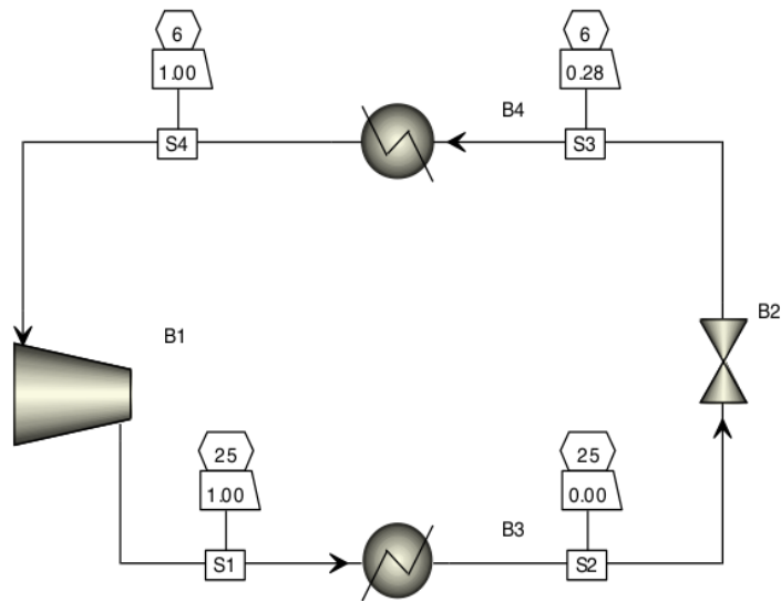
Figure 1. Single stage vapour compression cycle in Aspen-Plus
