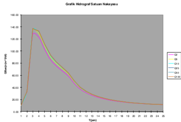
Figure 1. Hydrograph of water discharge in Samiran watershed
