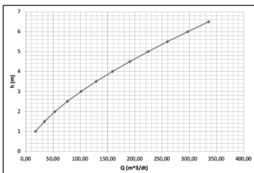
Figure 3. Relationship of water surface and water discharge
