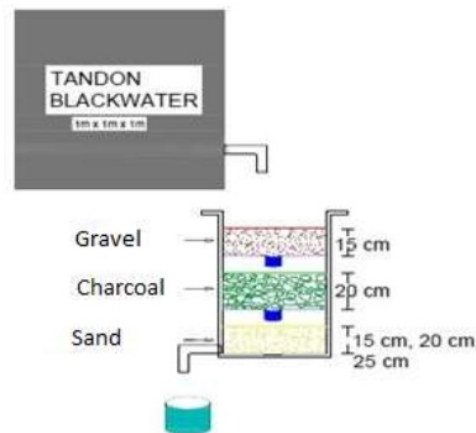
Figure 1. Stratified filter
