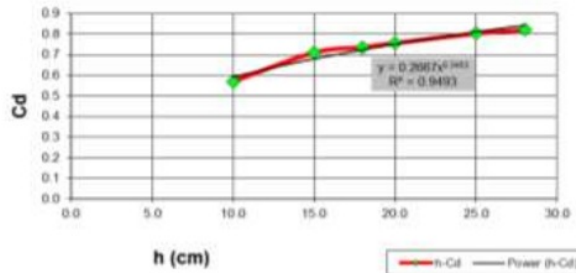
Fig. 4. Relationship between h and Cd in pipe 1
