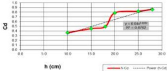
Fig. 5. Relationship between h and Cd in pipe 3
