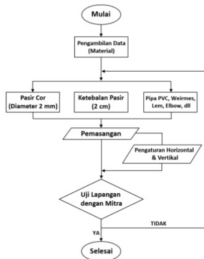
Gambar 4. Diagram Alir
