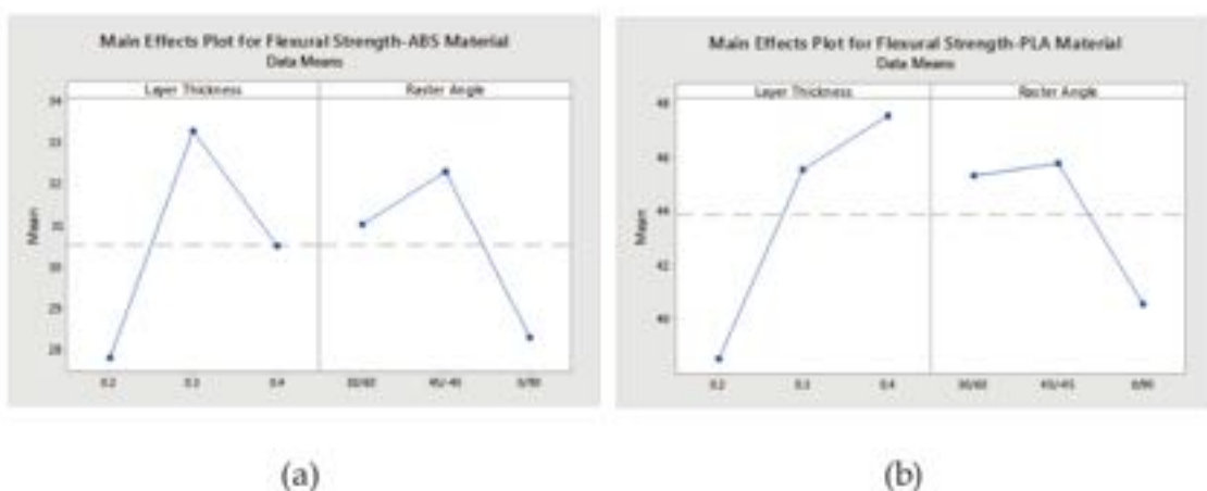
Figure 7: Main effect plot for flexural strength (a) ABS and (b) PLA specimen
