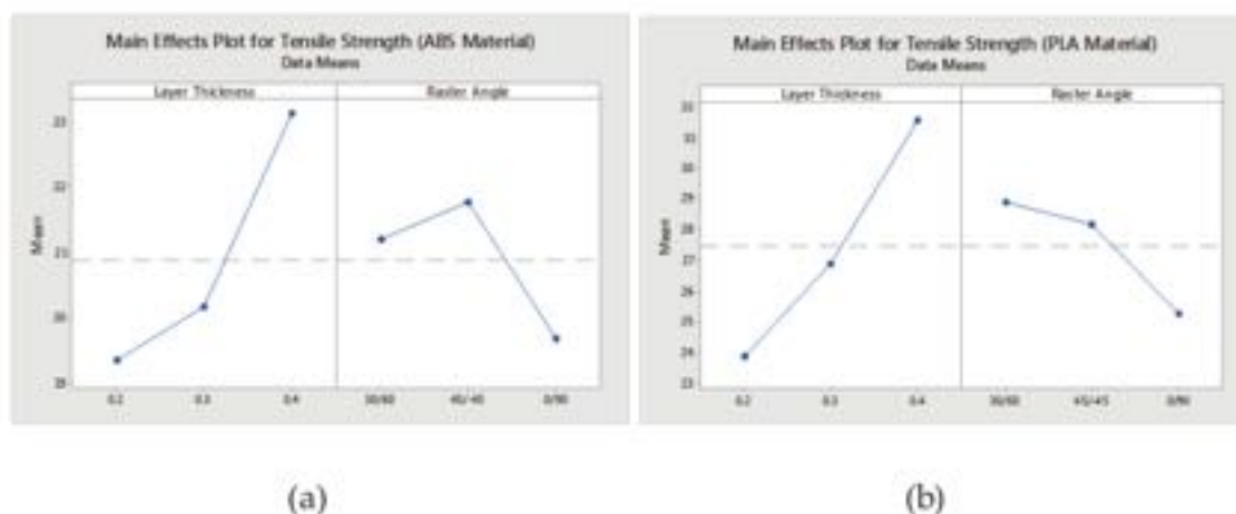
Figure 6: Main effect plot for tensile strength (a) ABS and (b) PLA specimen
