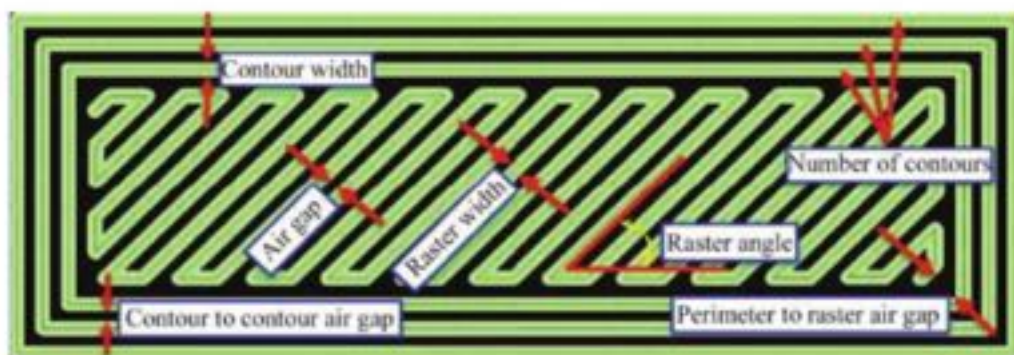
Figure 1: FDM tool path parameters [4]
