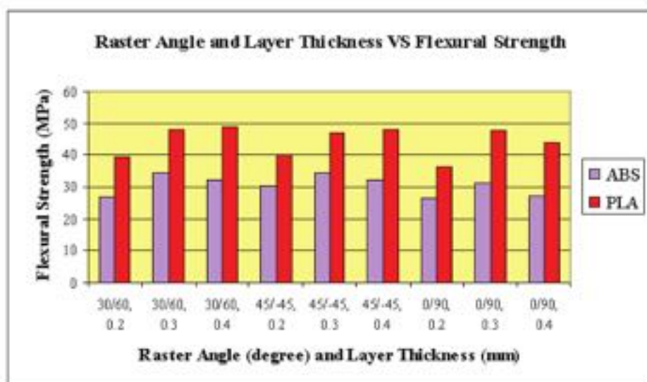
Figure 5: Flexural strength measurements of ABS and PLA specimens with various raster angle and layer thickness
