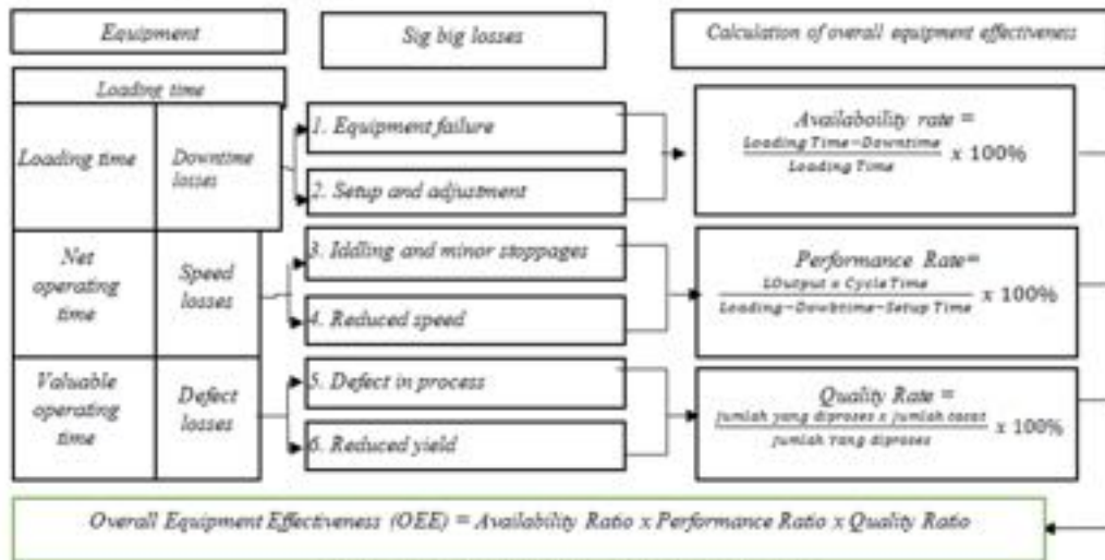
Fig 1:- Overall Equipment Effectiveness Process Source: Nakajima (1988)
