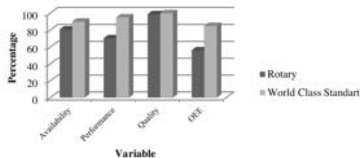
Fig 2:- Comparison Ratio Diagram of Rotary Machine
