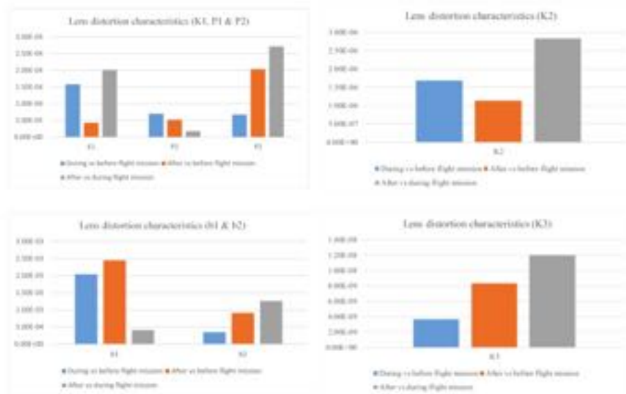
Figure 6: Lens distortion variations of the Lens before, during, and after the flight missions respectively; Deviations in lens distortion parameters between two epochs.
