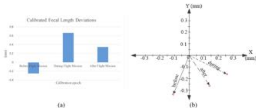
Figure 4: The IO parameters fluctuations prior to, during, and after the flight mission: (a), fixed focal length lens instabilities, (b), principal points instabilities.
