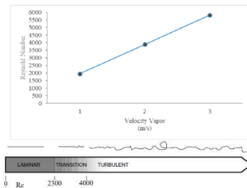
Fig 7. Graph of vapor velocity towards Reynold Number
