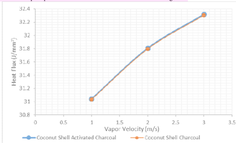
Fig 6. Heat Flux Chart
