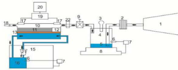
Fig 2. Research Tools Design
