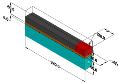
Fig 4. Test Section Design
