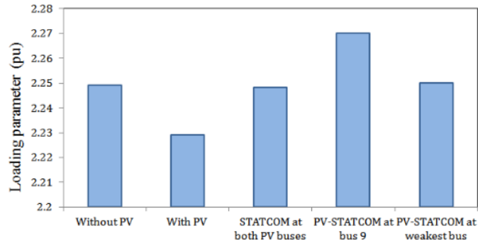
Figure 10. System loading margins for STATCOM placements.
