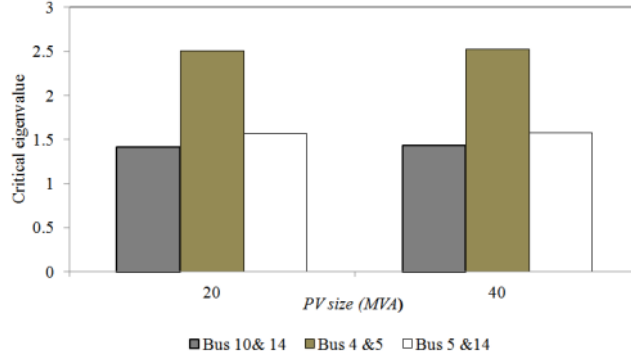
Figure 7. Effect of dispersed PV penetration on the degree of stability.
