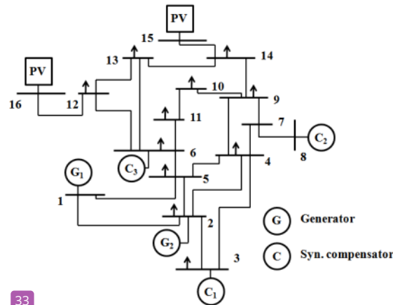
33 Figure 3. Single-line diagram of IEEE-14 bus test system.
