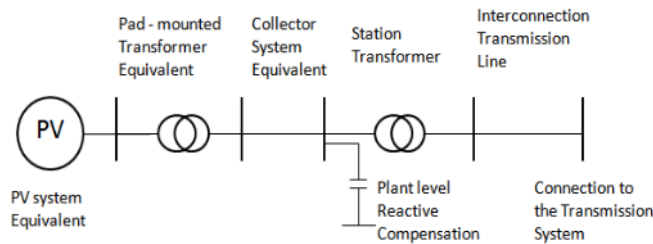
Figure 4. Schematic diagram of an aggregated PV generator.
