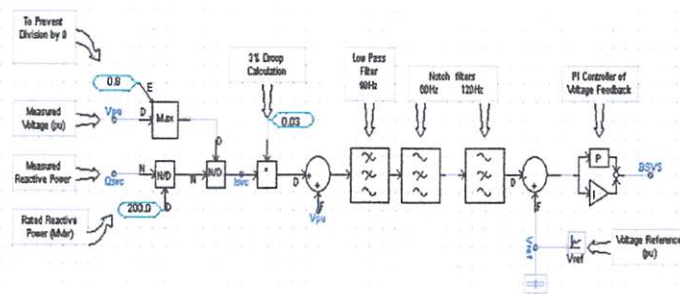
Gambar 3.16 Blok control PI
