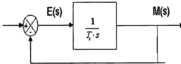
Gambar 3.13 Blok Diagram Kontroler Integral
