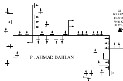
Gambar. 1. Single Line Diagram Feeder Ahmad Dahlan 20/0,4 kV
