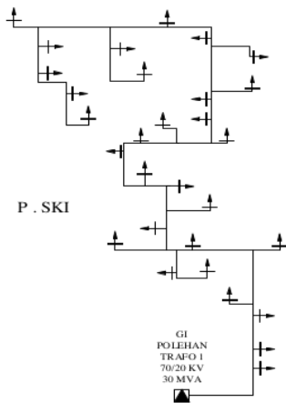
Gambar. 3. Single Line Diagram Feeder SKI 20/0,4 kV
