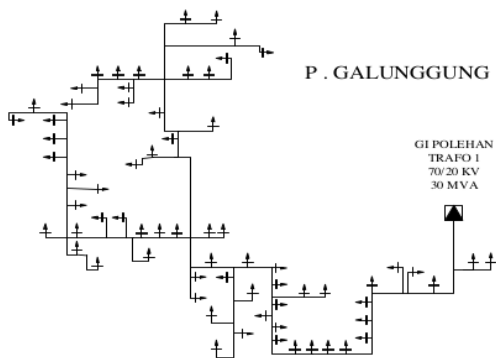
Gambar. 2. Single Line Diagram Feeder Galunggung 20/0,4 kV
