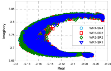
Fig. 12. Trajectories of inter area mode under hybrid MG active power uncertainty in area-2.
