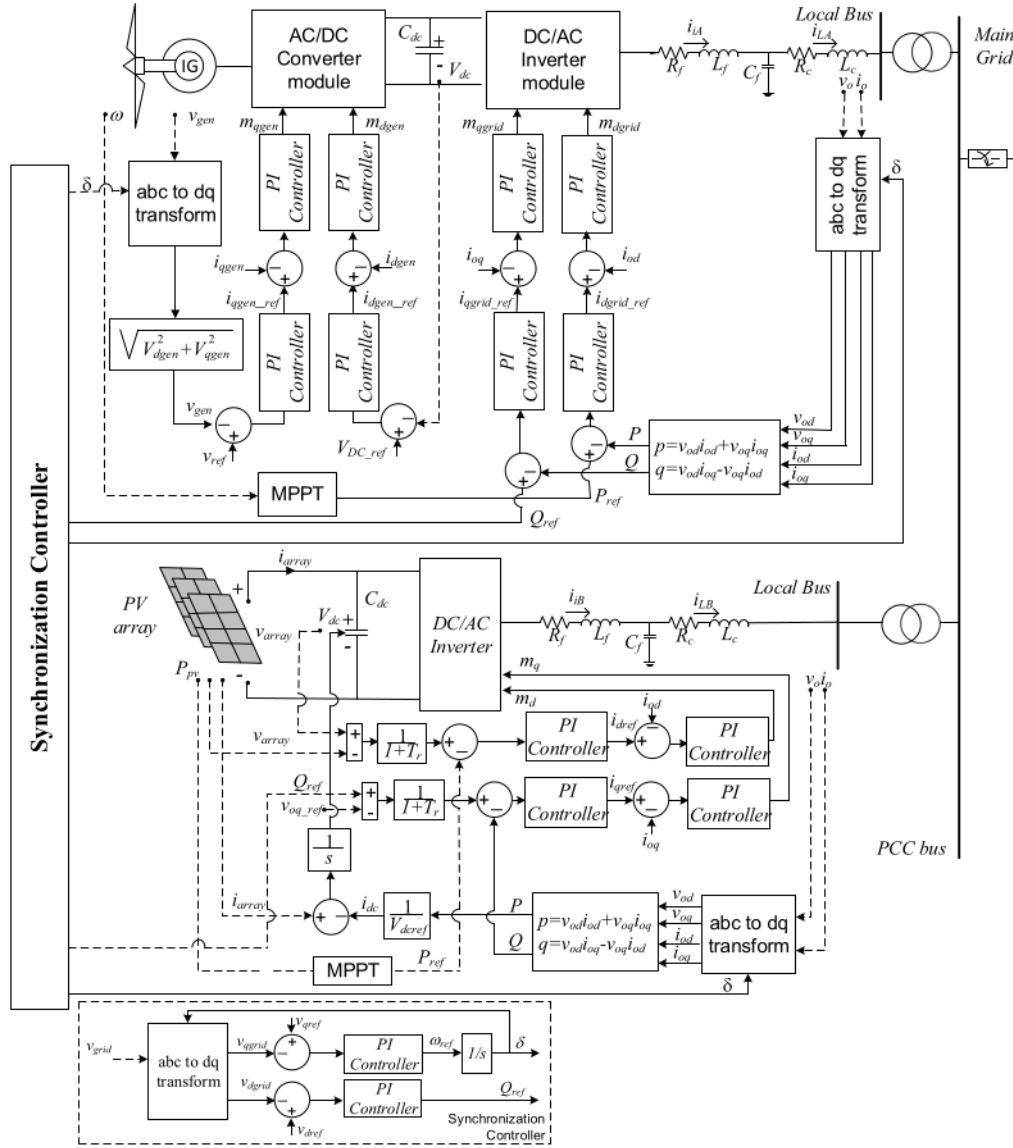
Fig. 2. Control system of each DG nit in the investigated MG system.
