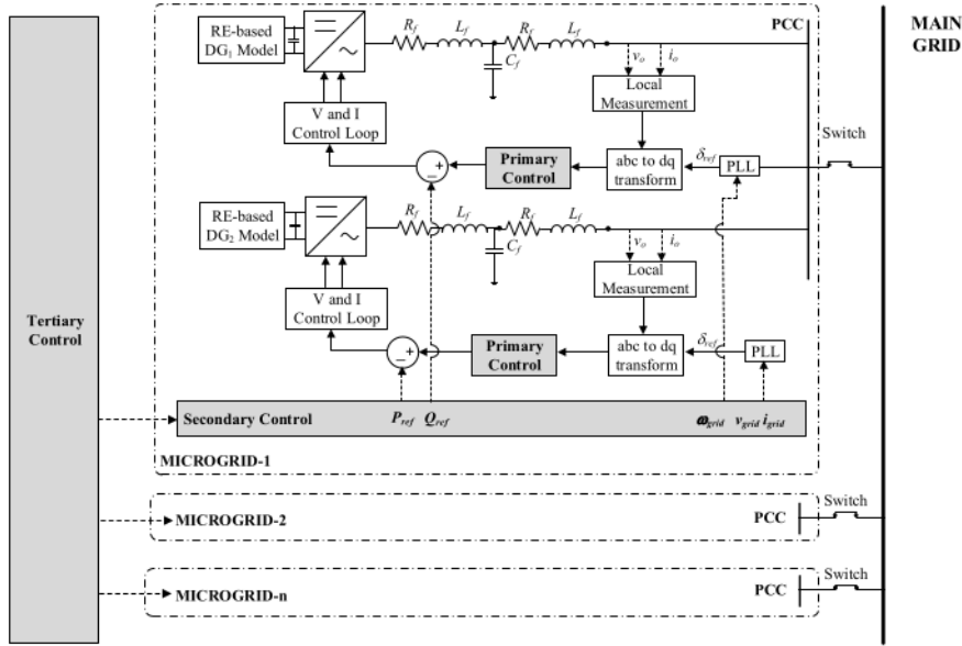
Fig. 1. Investigated hybrid microgrid system.
