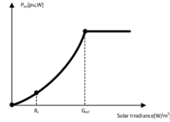
Fig. 3. PV power curve.
