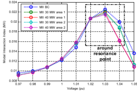
Fig. 19. MII values under increasing MG penetration.
