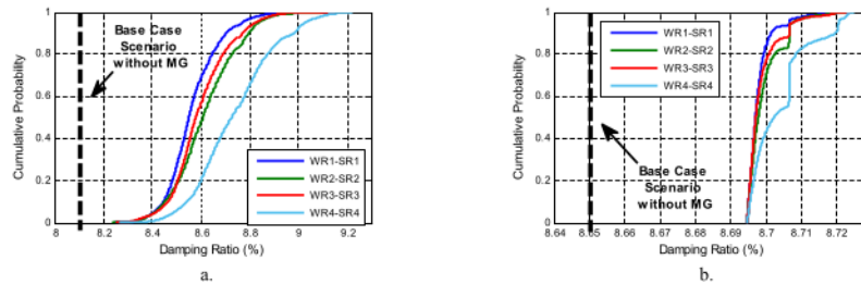
Fig. 9. CDF curve of damping ratio of local mode 1(a) and local mode 2(b) from two-area power system under hybrid MG power uncertainty in area 1.
