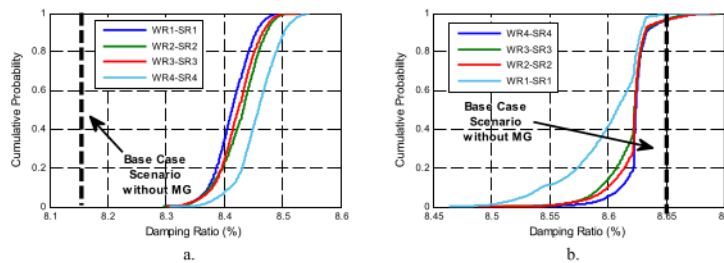
Fig. 13. CDF curve of damping ratio of local mode 1(a) and 2(b) from two-area power system under hybrid MG power uncertainty in area 2.
