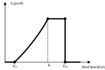
Fig. 4. Wind power curve.
