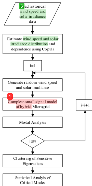
28 Gambar 2.2 Monte Carlo Simulation for Probability Small Signal Stability Analysis.
