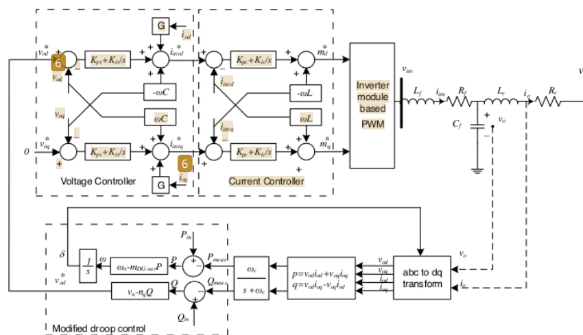
Figure 2.4 Modified droop control method.
