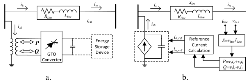
Gambar 3. Model STATCOM
