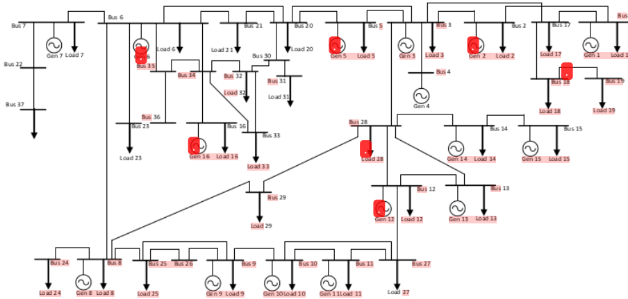
Gambar.4.1 Gambar One-Line Diagram Sistem Sulselbar 150 kV.
