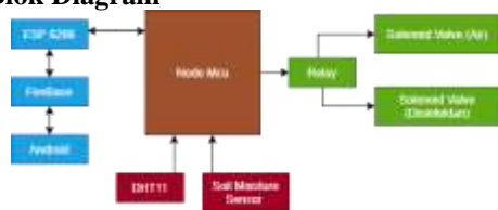
Gambar 3.1. Blok Diagram
