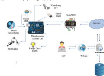
Gambar 1. Diagram block sistem
