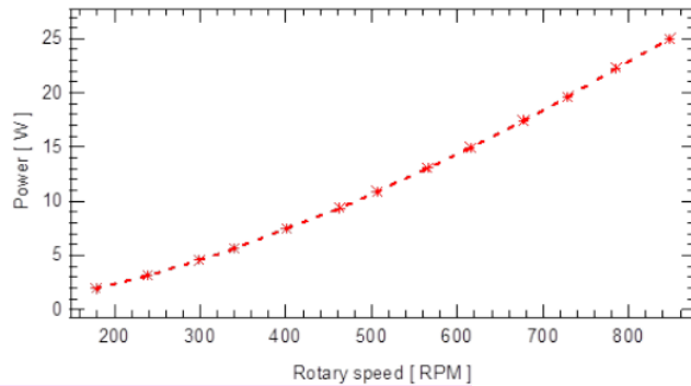
2 Figure 9 Correlation between output power and rotational speed.
