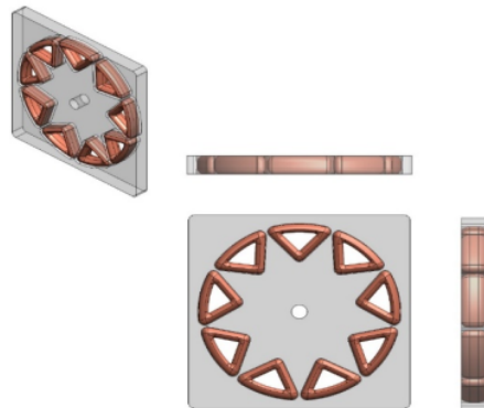
Figure 3 Stator design of double-sided axial flux permanent magnet generator.
