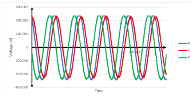
Figure 5 Three phase voltage output at frequency of 41.4 Hz.
