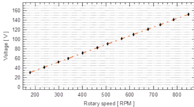
Figure 8 Correlation between rotational speed and DC voltage.
