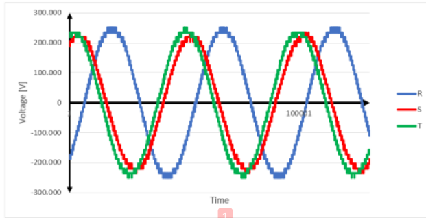
Figure 4 Three phase voltage output at frequency of 20.5 Hz.
