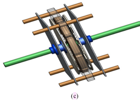
Figure 1 Design and experimental setup of double side axial flux permanent magnet generator: (a) diagram of proposed double side axial flux permanent magnet generator (b) experimental setup of double side axial flux permanent magnet generator (c) the design of double side axial flux permanent magnet generator
