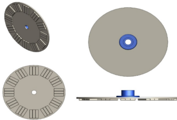
Figure 2 Design of double-side rotor in proposed axial flux generator.
