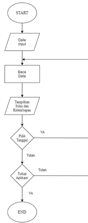
Gambar 9. Flowchart Web
