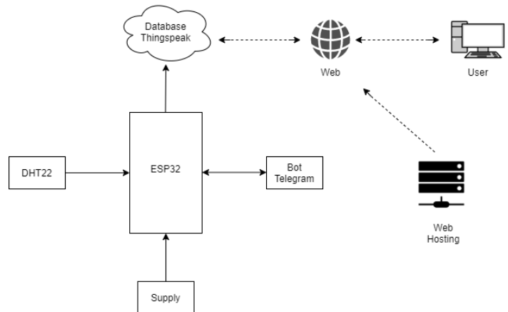
Gambar 7. Blok Diagram
