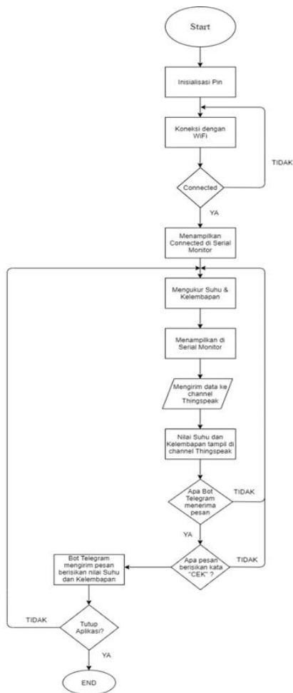
Gambar 8. Flowchart Alat
