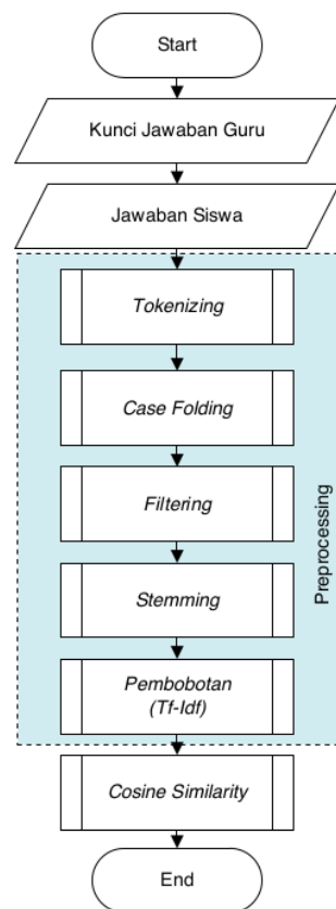
Gambar 1. Flowchart sistem
