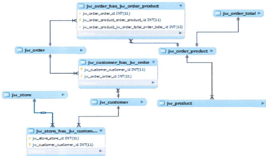
Gambar 3.5 Diagram Skema
