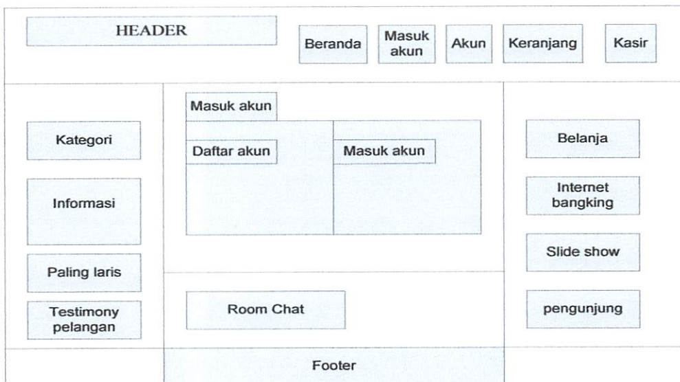
Gambar 3.9 Halaman login member
