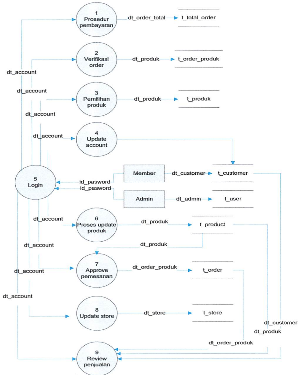
Gambar 3.3 DFD Level 1
