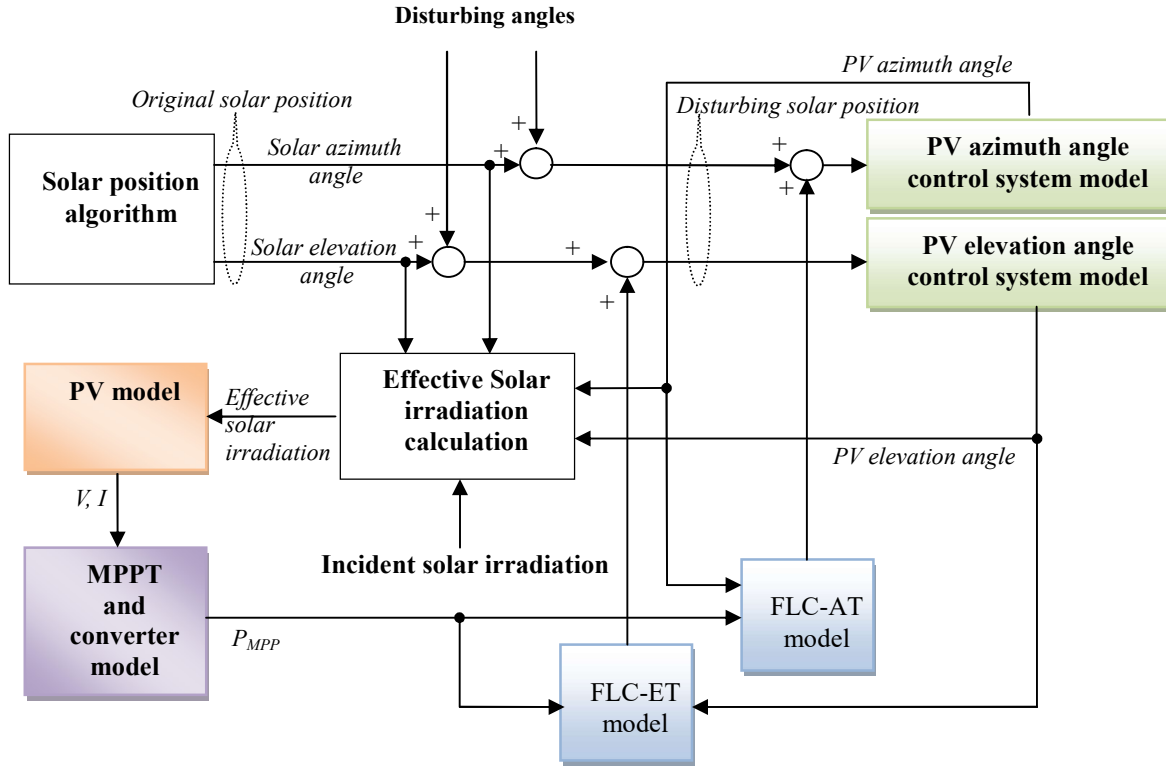
FIGURE 4. Integrated solar tracker and MPPT model.
