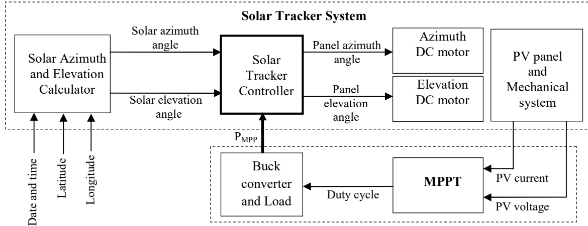
FIGURE 1. Architecture of proposed system.
