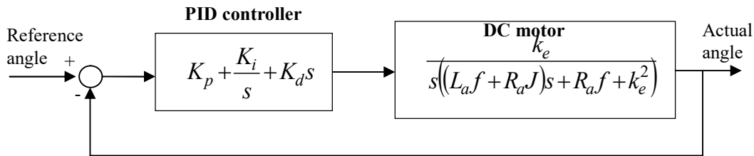
FIGURE 5. PID controller and DC motor model.
