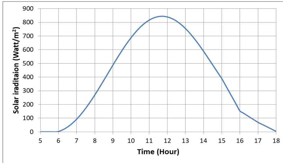
FIGURE 6. Profiles of solar irradiation.
