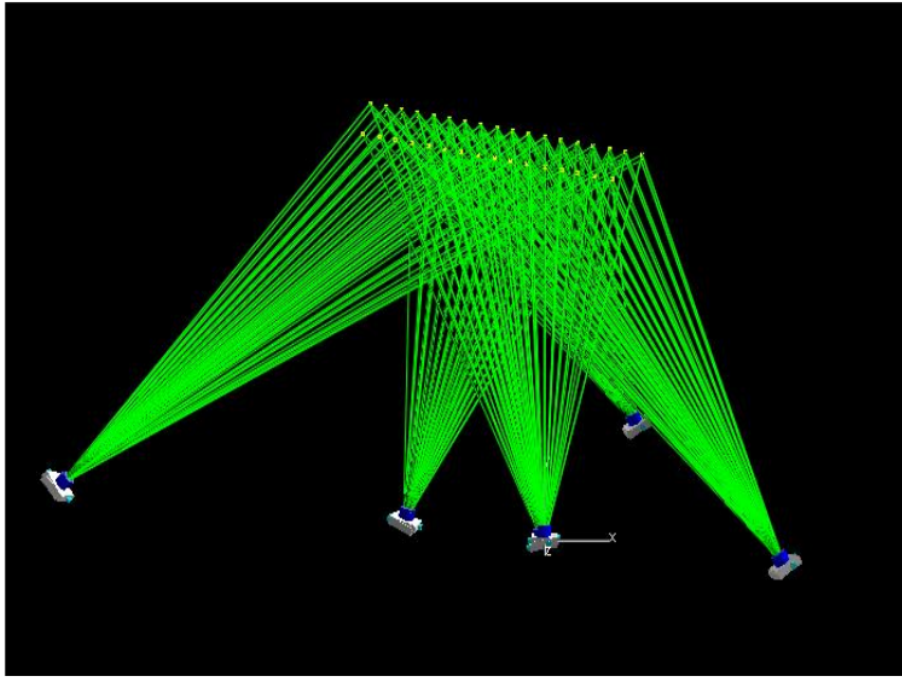
Gambar 7. Ilustrasi proses bundle adjustment (Wolf & Dewitt, 2014)
