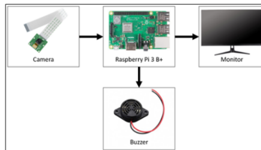
Figure 2. Hardware design
