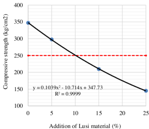
Fig.6. The relationship between the addition of Lusi material and the compressive strength of concrete
