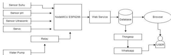
Gambar 9. Blok Diagram
