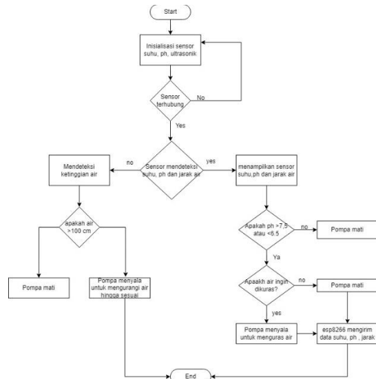
Gambar 7. Flowchart Sistem
