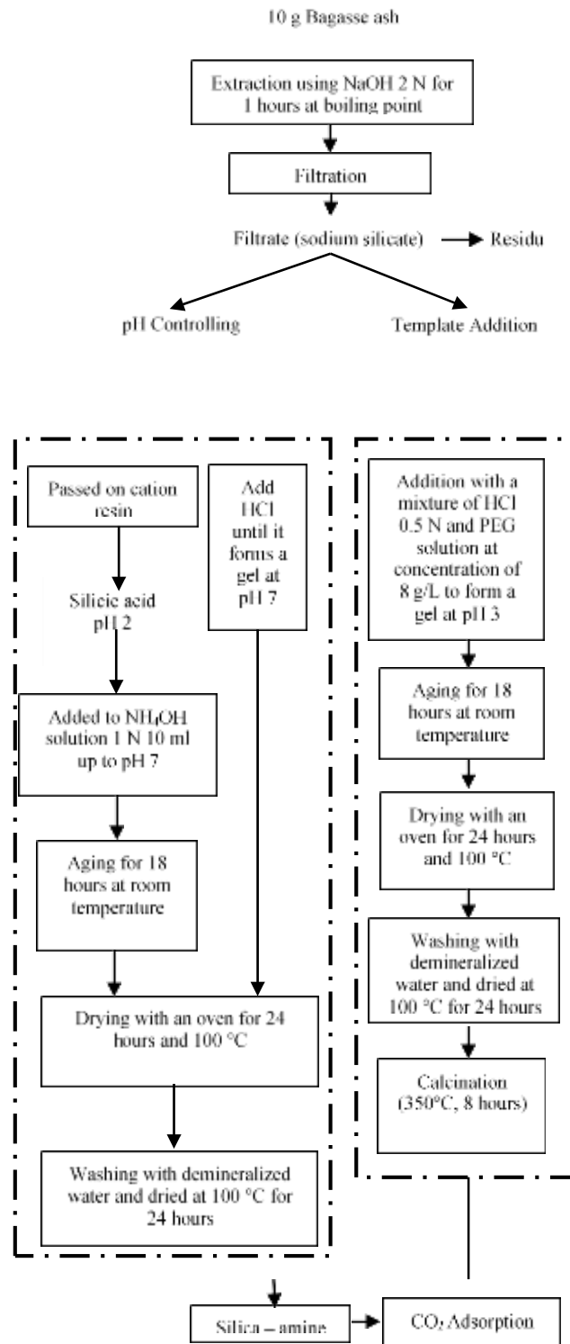
Fig. 1. Flow chart of silica-amine synthesis process
