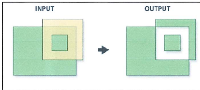
Gambar 2.10 Fungsi Subtract
