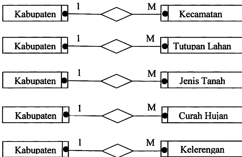
Gambar 3.15 Diagram Obligatory/non
