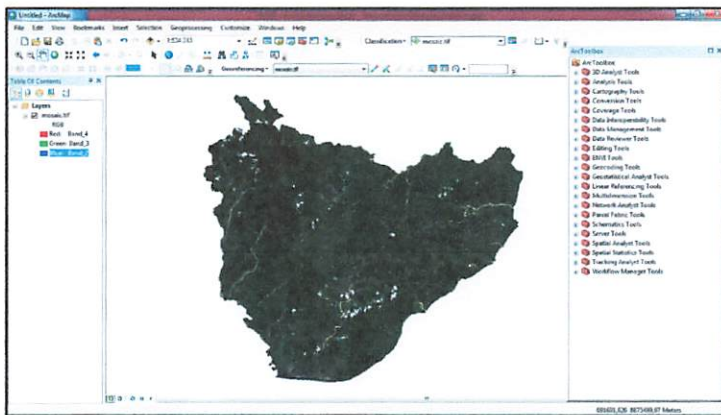
Gambar 3.11 Hasil Cropping
