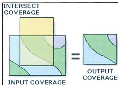
Gambar 2.8 Fungsi Intersect
