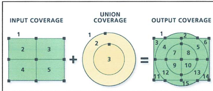
Gambar 2.9 Fungsi Union
