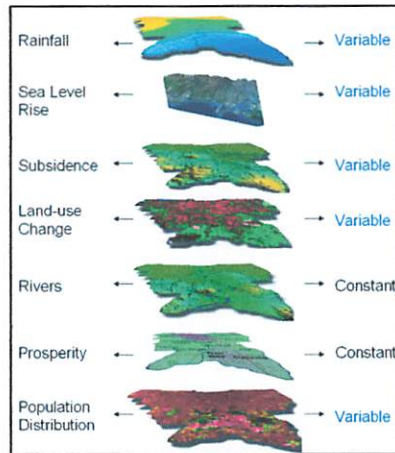
Gambar 2.7 Analisis Overlay
